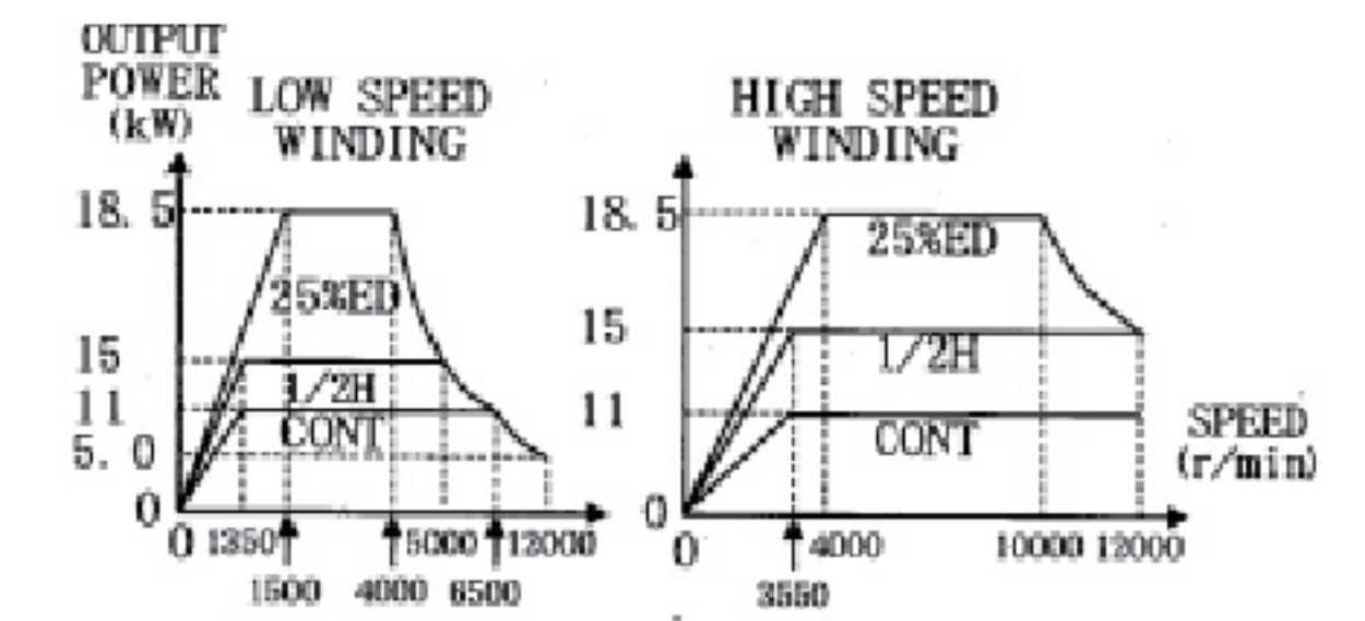
OUTPUT POWER - SPEED CHARACTERISTIC NORMAL
