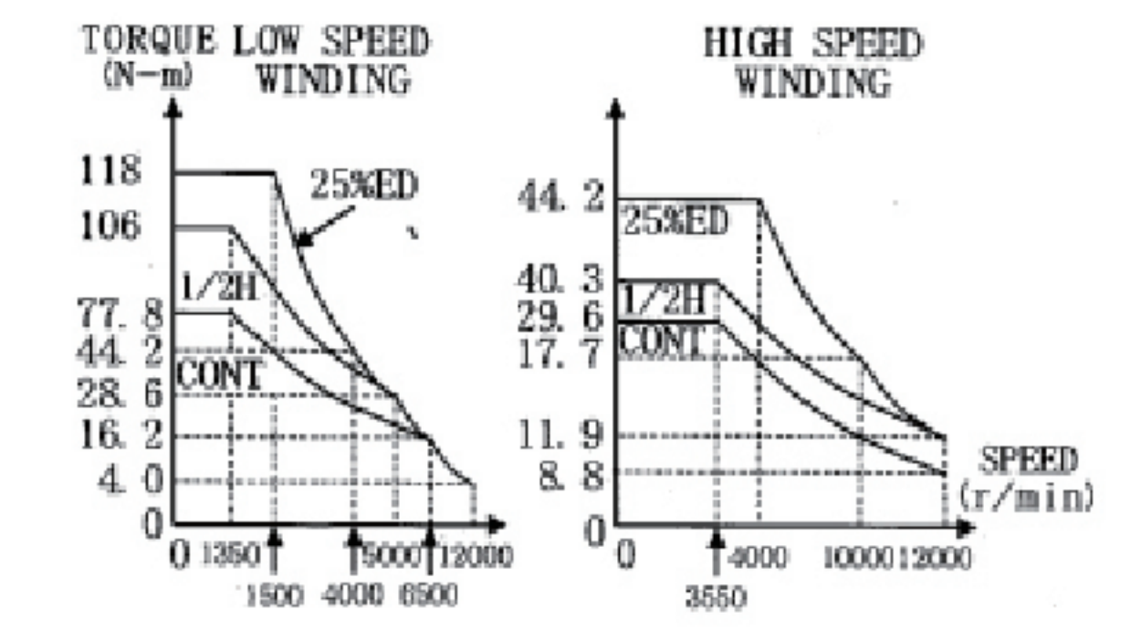
TORQUE - SPEED CHARACTERISTIC NORMAL
